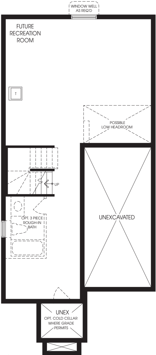
BASEMENT ELEVATION 'A'
