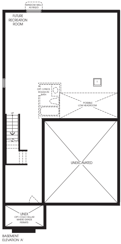
BASEMENT ELEVATION 'A'
