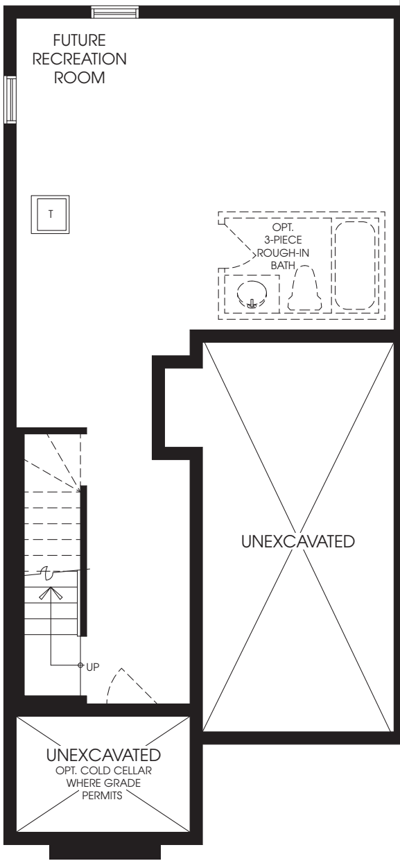
BASEMENT ELEVATION 'A1' & 'A2'
