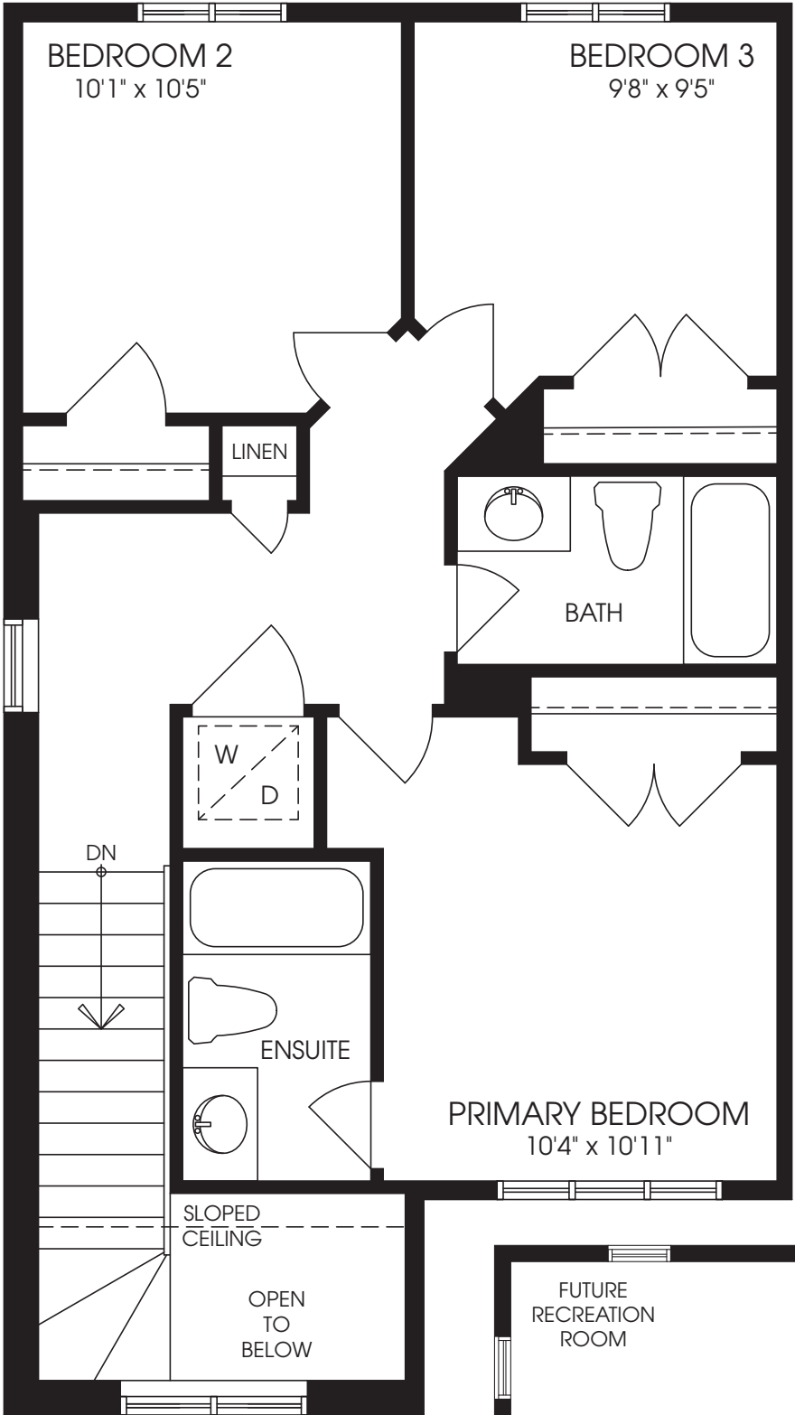
SECOND FLOOR ELEVATION 'A1'
