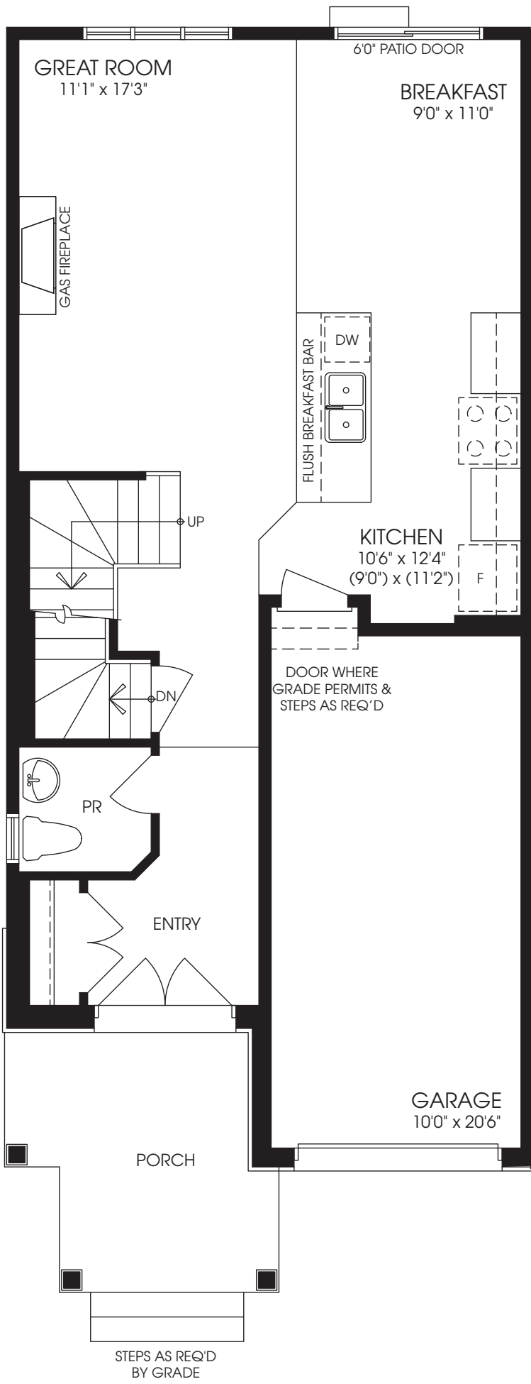
MAIN FLOOR ELEVATION 'A1' & 'A2'
