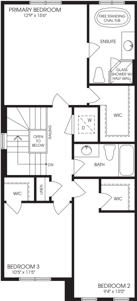
OPTIONAL SECOND FLOOR W/ LARGE ENSUITE ELEVATION 'A'
