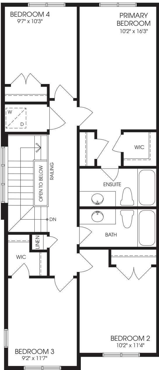
OPTIONAL SECOND FLOOR W/ 4 BEDROOMS ELEVATION 'A'
