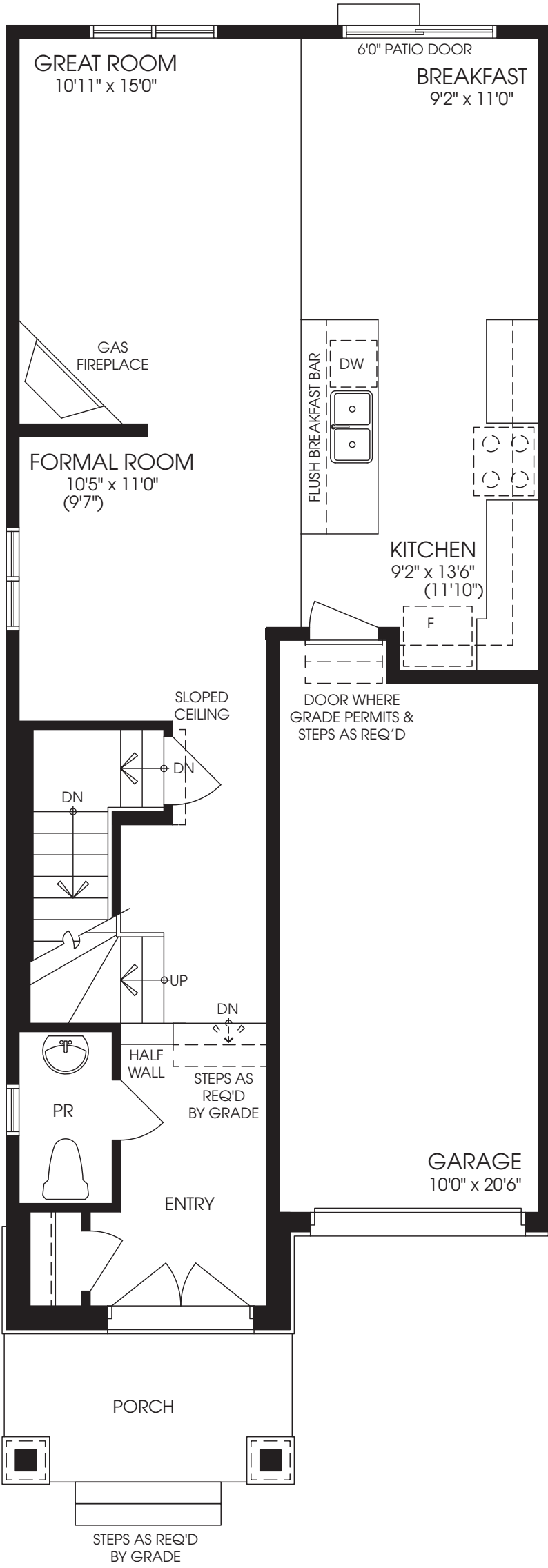
MAIN FLOOR ELEVATION 'A'
