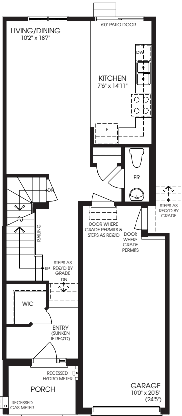
OPT. MAIN FLOOR ELEVATION 'A1'
