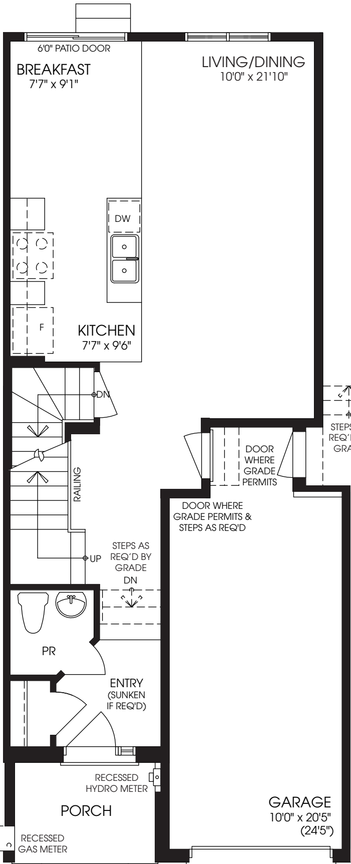
MAIN FLOOR ELEVATION 'A1'
